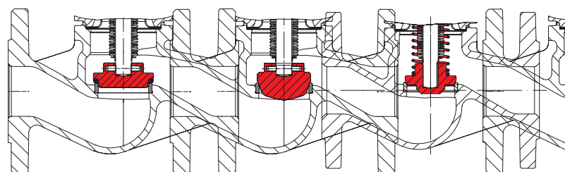
Regulation plug
