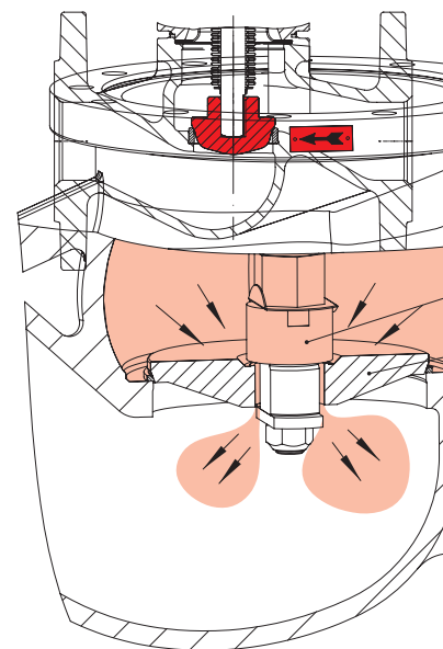
Regulation plug
